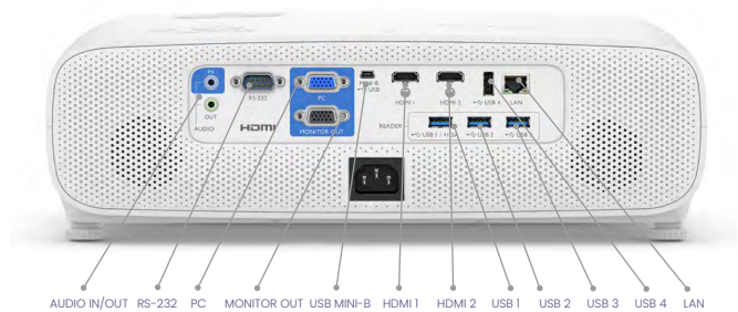
AUDIO IN/OUT RS-232 PC MONITOR OUT USB MINI-B HDMI 1 HDMI 2 USB 1 USB 2 USB 3 USB 4 LAN
