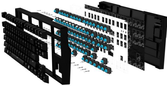
Keyboard design combining Cherry MX Switches, Metal Plate and Bright LEDs.
